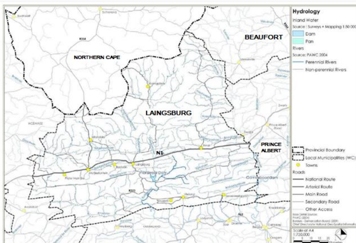
Figure 6.1 Laingsburg Hydrology: Rivers (Source: LLM SDF; 2012)
