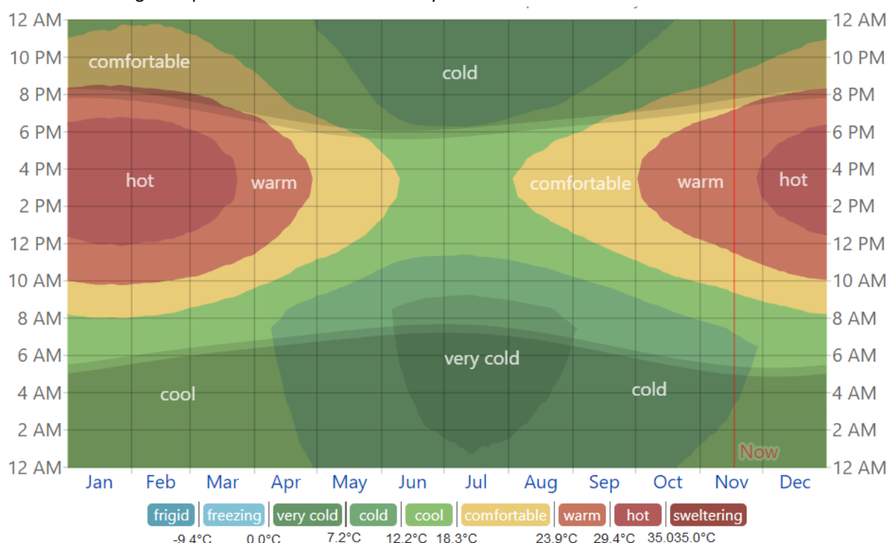
Figure: Average Hourly Temperature in Laingsburg
